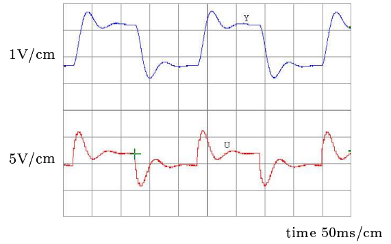
Figure 9. Response (Y) and control signal (U) from object II with direct STR without zeros cancellation.
