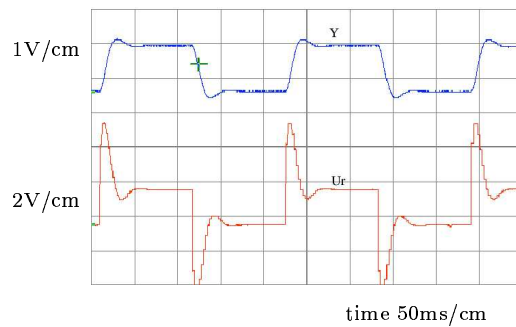
Figure 11. Object II with direct STR.
